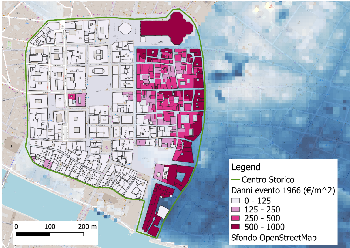
FIGURE 16: FLOOD LOSSES FOR AN EVENT SIMILAR IN MAGNITUDE TO THE 1966 FLOOD
